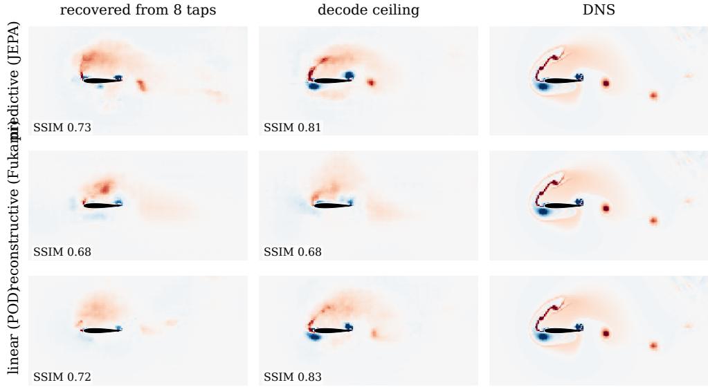
Figure 23. Flow recovered from eight wall-pressure taps on the representative held-out encounter of figure 11, at the impact-side frame, one row per family. Columns: the field decoded from the pressure-recovered coefficient state, the decode ceiling (the same decoder applied to the encoded state, no pressure step), and the simulation; per-panel structural similarity annotated. The comparison is within each row, since the decoders' ceilings differ (§5.3); the ceiling-to-recovered gap is the cost of the pressure step.
