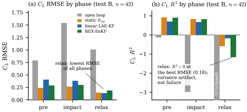
Figure 13. Phase-resolved lift tracking on the in-distribution test set ( n = 42 encounters, K = 8 taps, delay 10, N = 64 members, every-frame pressure). Lift error per phase in physical units (a) and in R^2 (b) at the val-calibrated band: the relaxation R^2 collapse is a variance artifact, the physical error the honest phase metric. The estimator ladder, its noise calibration and the fixed-lag smoother are in appendix C (figure 27).
