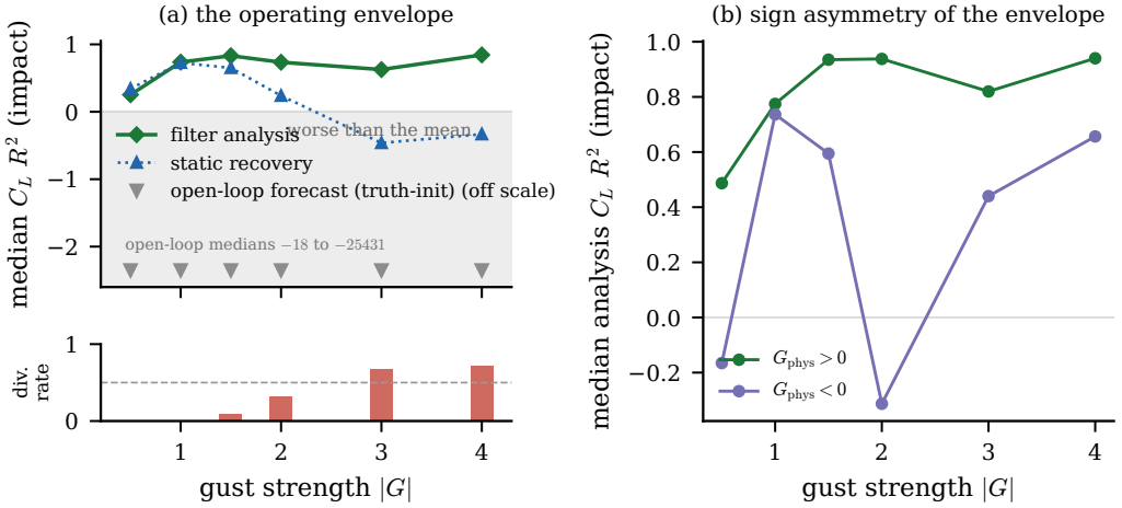
Figure 12. The gust-intensity operating envelope. (a) Median analysis lift closure ( R^2 , impact window) against gust strength for the frozen filter, the static single-frame recovery, and the truth-initialised open-loop forecast, with the filter consistency-failure rate as the strip beneath; the shaded band marks closure worse than predicting the encounter mean, and the open-loop forecast lies off the scale below it. (b) The same filter closure resolved by the physical sign of the gust, showing the wider usable envelope of the positive gusts.
