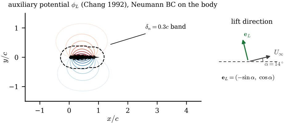
Figure 19. The Chang auxiliary potential \phi_L of equation (3.1) on the cache grid (contours), the feathered \delta_n = 0.3c supervision band (dashed) and the airfoil footprint; the inset shows the lift direction \mathbf{e}_L against the inclined freestream at \alpha = 14^\circ .
