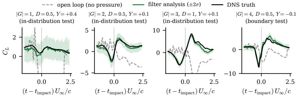
Figure 15. C_L estimation before and after impact across the gust-intensity envelope, on the wake-supervised predictive state ( d = 32 ) under the two-stage filter of §3.3.3: inside the impact window the members are advanced by the direct multi-horizon forecaster’s median forecast with its quantile band as state-dependent process noise (production scale c = 1.77 , validation-calibrated) and corrected by the encoded pressure observation; outside it, by the matched transformer with the tap-space update. Eight wall-pressure taps, N = 64 members; the lift probe that produces the plotted read-out never enters the innovation. Band: \pm 2 ensemble standard deviations; grey, the same stage-scheduled forecast models rolled deterministically without pressure. One representative encounter per |G| stratum (median impact closure on the frozen two-stage filter records; in-distribution test set for |G| \leq 3 , boundary test set at |G| = 4 , where this filter posts no divergent encounter). The analysis tracks the lift through impact and relaxation at every intensity; the open loop loses the transient.
