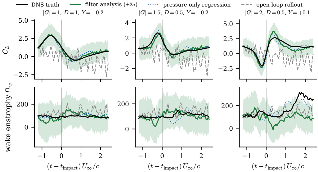
Figure 14. The estimator tracks the encounter from wall pressure alone. Columns are representative held-out encounters at |G| = 1, 1.5 and 2 ; rows are the lift coefficient and the wake enstrophy. Each panel shows the DNS truth, the filter analysis with its \pm 2\sigma ensemble band, the pressure-only regression, and the open-loop rollout; the vertical line marks impact. The filter follows the load through impact and relaxation where the open-loop forecast loses it and the pressure-only regression goes stale.
