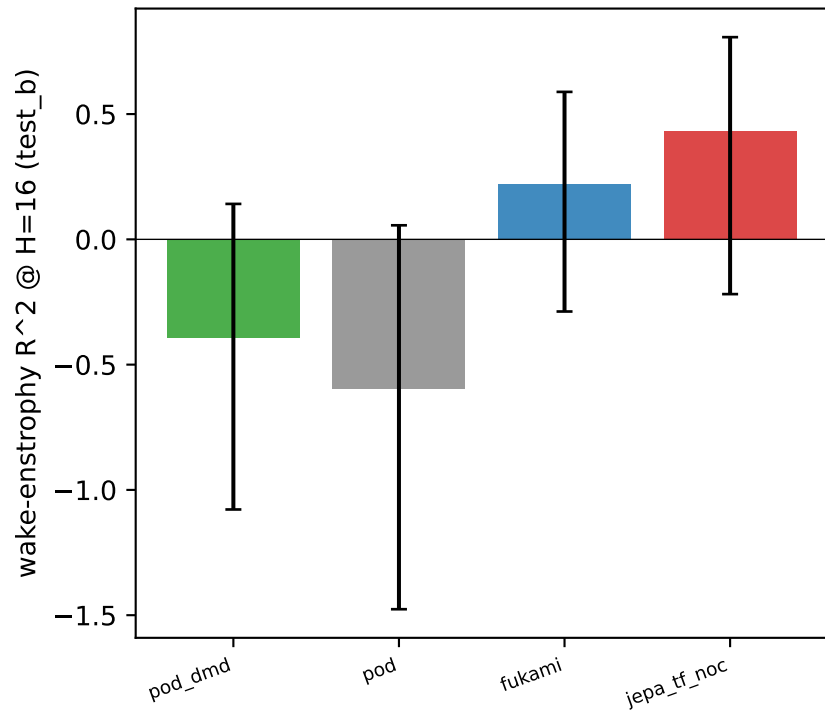
DMD rung vs learned predictors (forecast)
