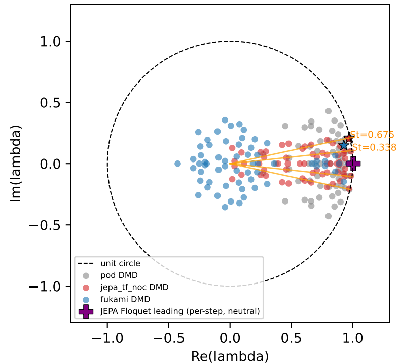
Latent spectrum (Baseline limit cycle)
