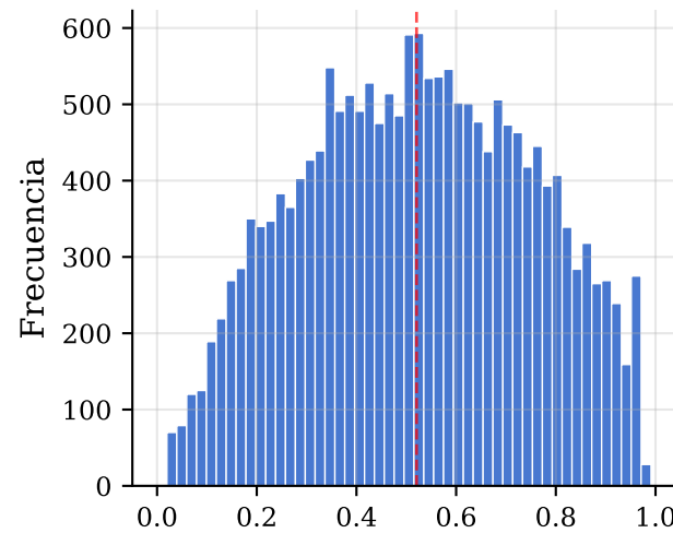
valence
