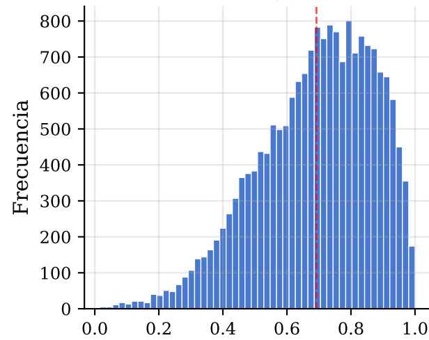
speechiness
