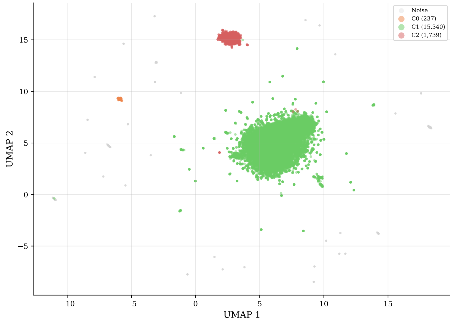
Clusters HDBSCAN K = 3 --- Semántico (UMAP 30D)
