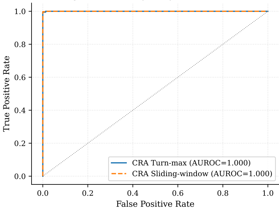
Fig. 5 — CRA Trajectory ROC on CoSafe
