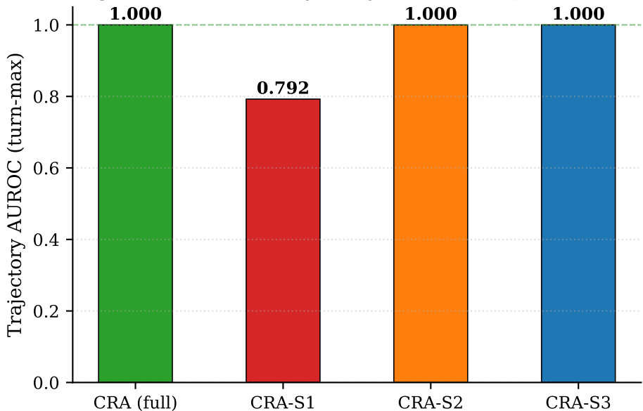
Fig. 6 — Ablation: Trajectory AUROC Drop on CoSafe
