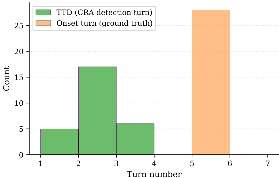
Fig. 8 — TTD vs Onset-Turn Distribution (CoSafe, threshold=0.45)
