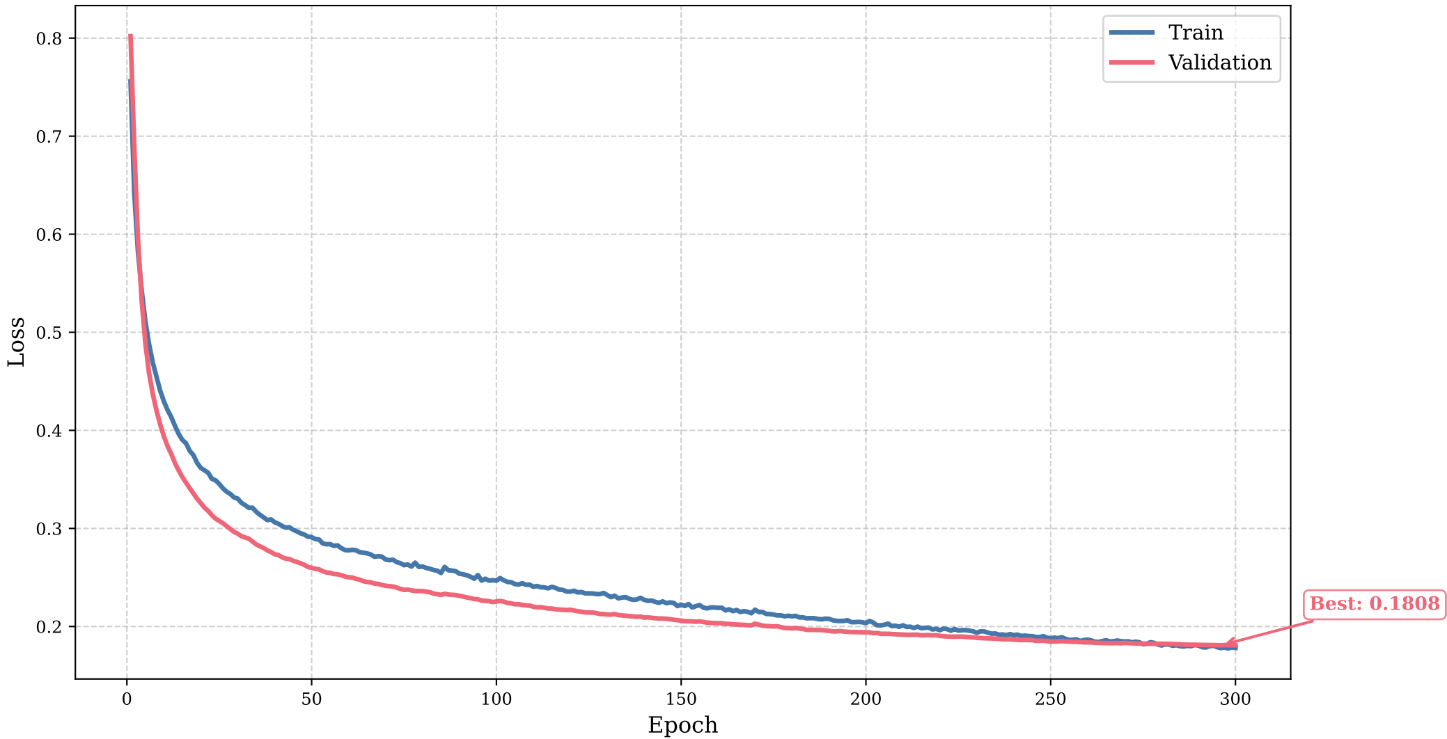
Dice Loss
