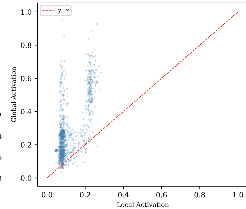
Per-Position Correlation
