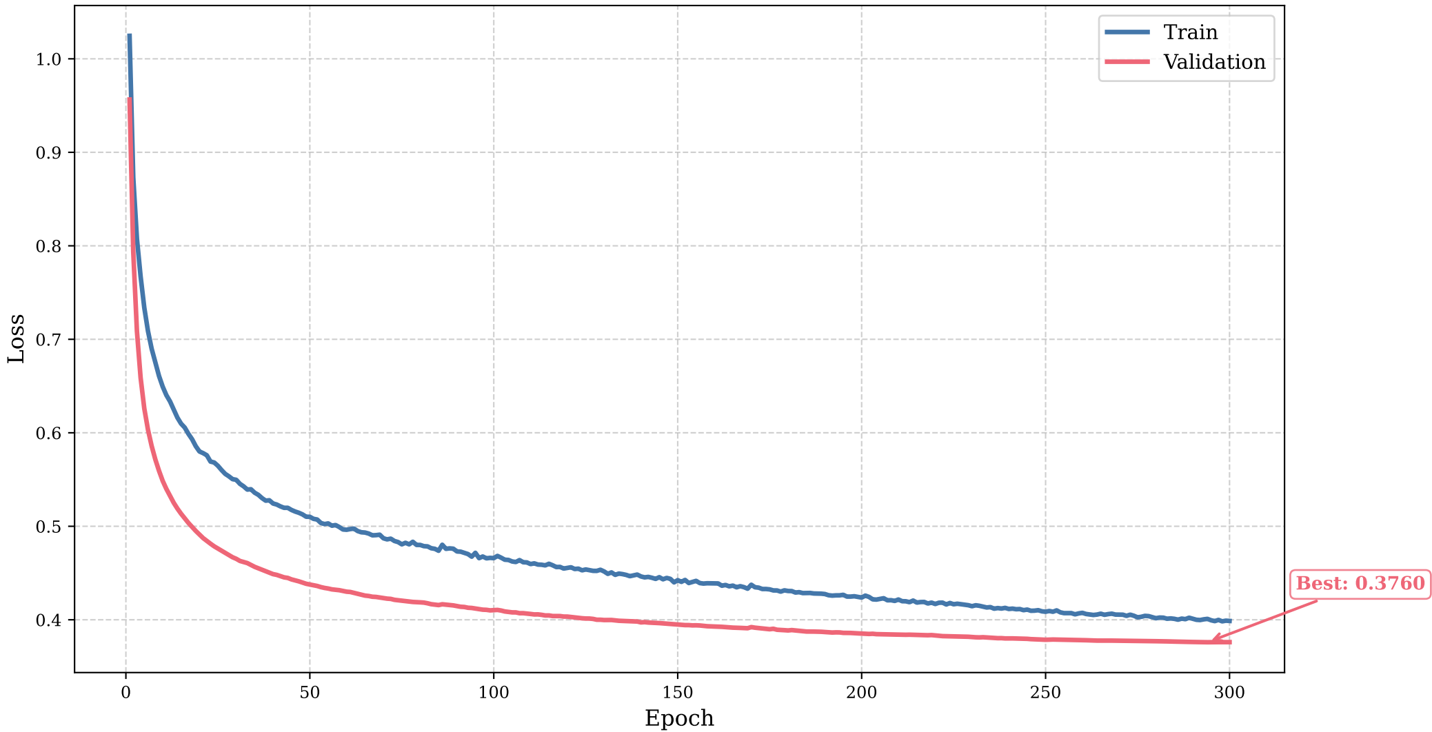
Combined Loss (CE + Dice)
