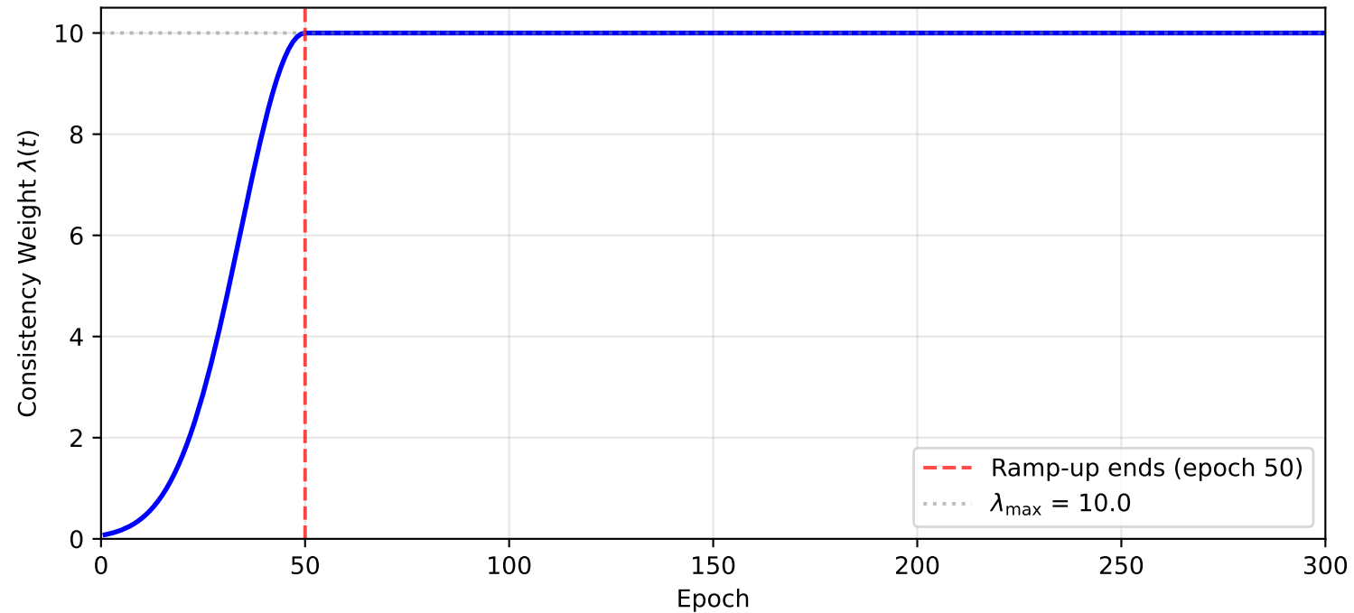
Sigmoid Ramp-up Schedule for Consistency Weight
