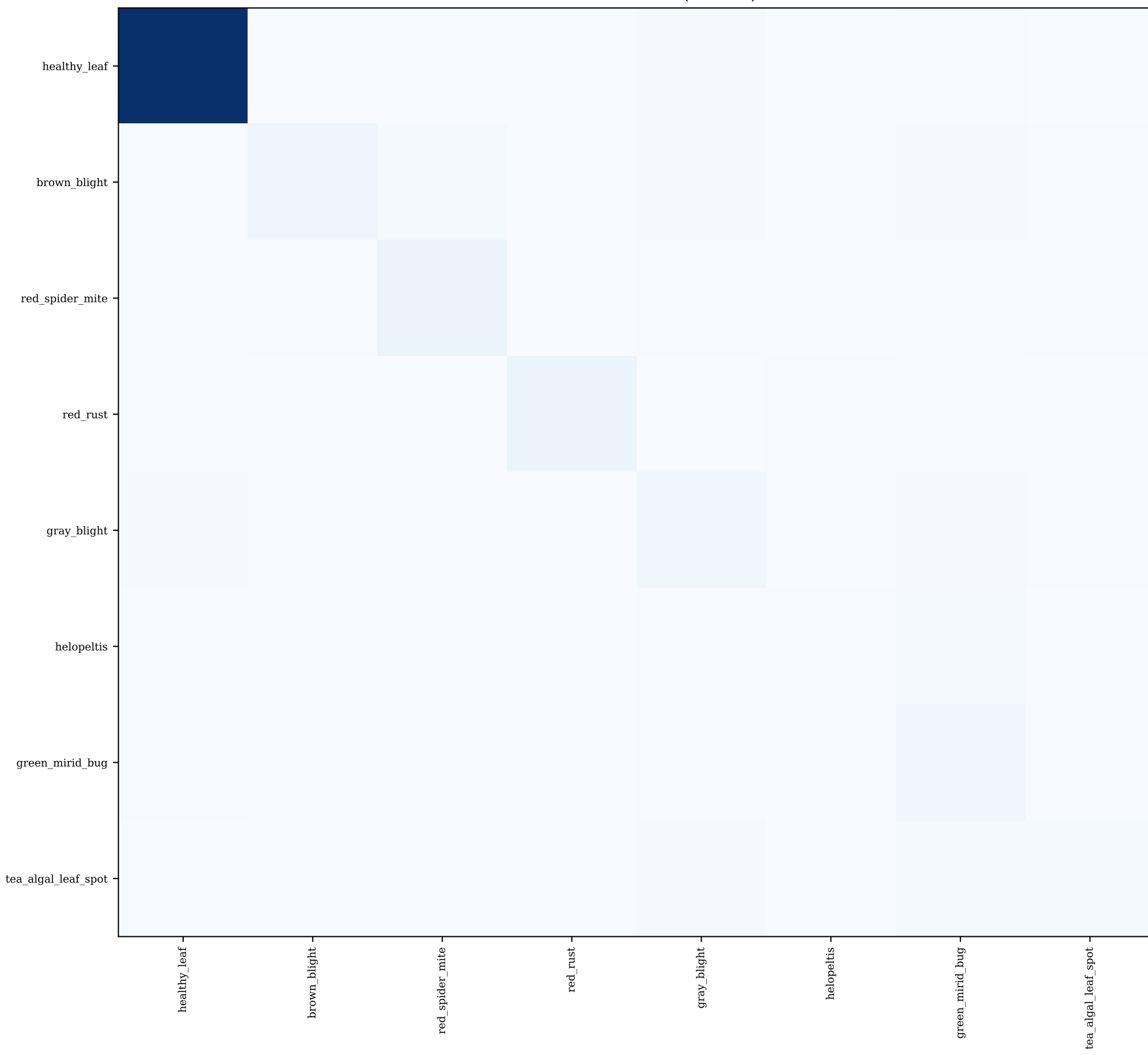
Confusion Matrix (counts)
