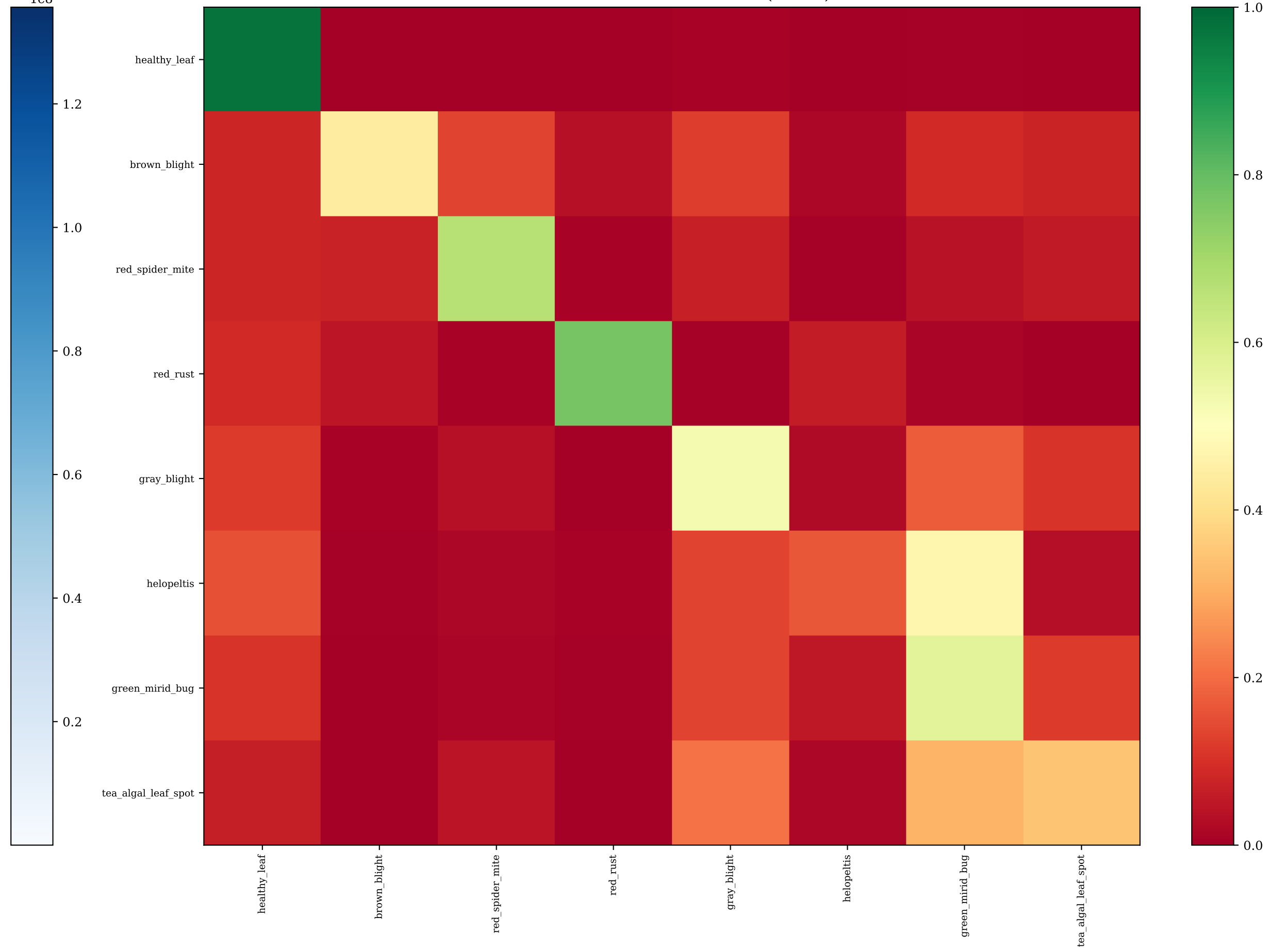
Normalised Confusion Matrix (Recall)
