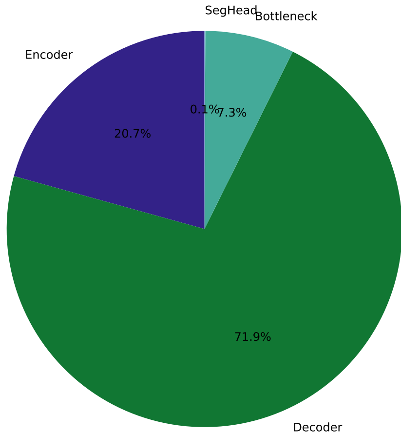
FLOPs Distribution | UNet-lite
