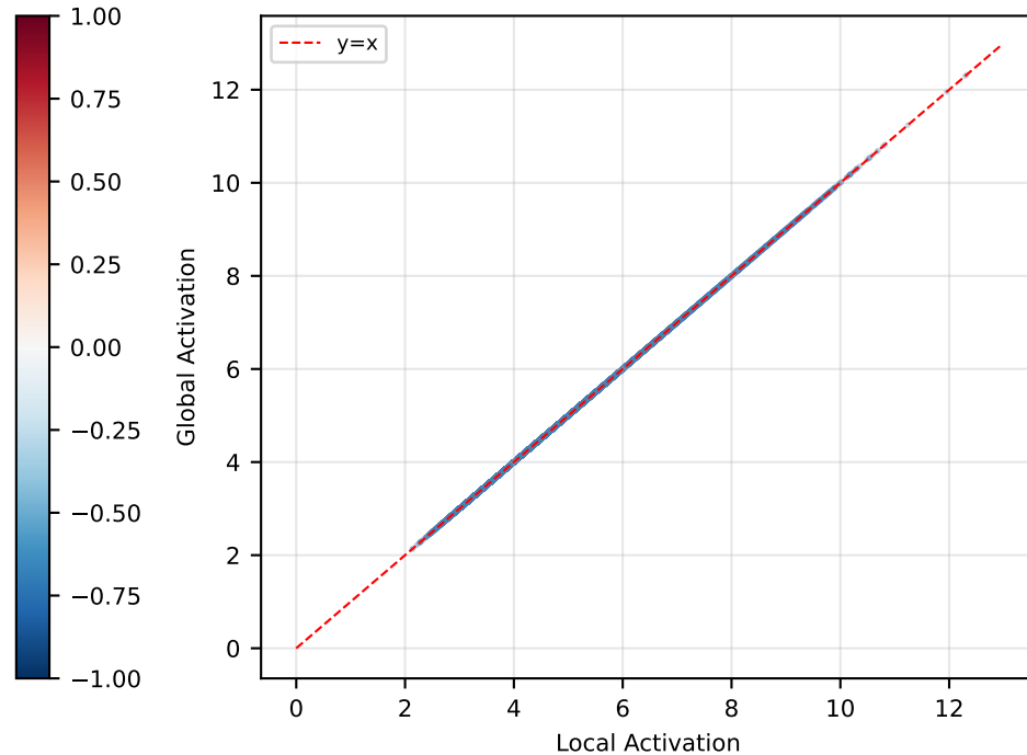
Per-Position Correlation
