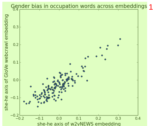
Figure 4: Comparing the bias of two different embeddings—the w2vNEWS and the GloVe web-crawl embedding. In each embedding, the occupation words are projected onto the she-he direction. Each dot corresponds to one occupation word; the gender bias of occupations is highly consistent across embeddings (Spearman \rho = 0.81 ).
