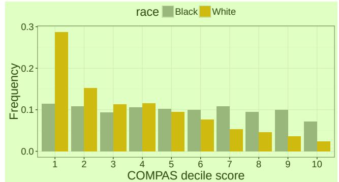
Figure 3: COMPAS decile score histograms for Black and White defendants. Cohen's d = 0.60 , non-overlap d_{\text{TV}}(f_b, f_w) = 24.5\% .
