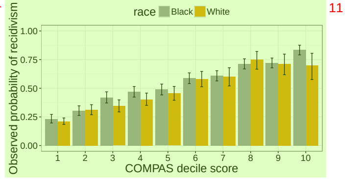
Figure 1: Plot shows \mathbb{P}(Y = 1 \mid S = s, R) for the COMPAS decile score, with R \in \{\text{Black}, \text{White}\} . Error bars represent 95% confidence intervals.
