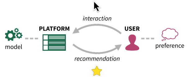
Figure 1: The feedback loop between user behavior and algorithmic recommendation systems. Confounding occurs when a platform attempts to model user behavior without accounting for recommendations. User preferences act as confounding factors, influencing both recommendations (through past interactions) and current interactions.
