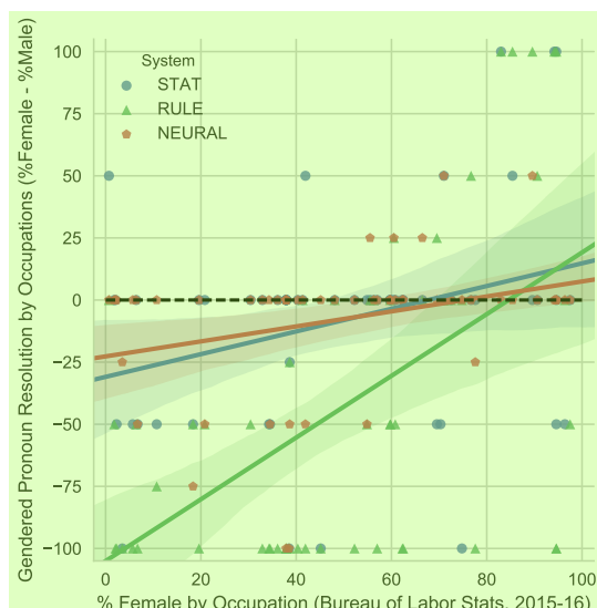
Figure 4: These two plots show how gender bias in coreference systems corresponds with occupational gender statistics from the U.S Bureau of Labor Statistics (left) and from text as computed by Bergsma and Lin (2006) (right); each point represents one occupation. The y-axes measure the extent to which a coref system prefers to match female pronouns with a given occupation over male pronouns, as tested by our Winogender schemas. A value of 100 (maximum female bias) means the system always resolved female pronouns to the given occupation and never male pronouns (100% - 0%); a score of -100 (maximum male bias) is the reverse; and a value of 0 indicates no gender differential. Recall the Winogender evaluation set is gender-balanced for each occupation; thus the horizontal dotted black line ( y=0 ) in both plots represents a hypothetical system with 100% accuracy. Regression lines with 95% confidence intervals are shown.
