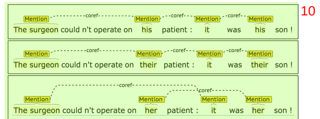
Figure 1: Stanford CoreNLP rule-based coreference system resolves a male and neutral pronoun as coreferent with "The surgeon," but does not for the corresponding female pronoun.
