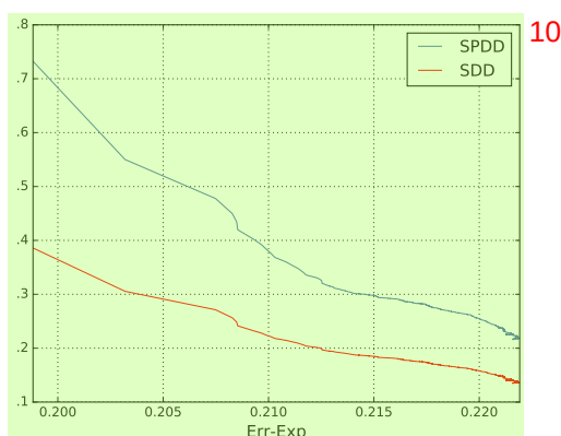
Figure 2: Err-Exp v.s. SDD, Err-Exp v.s. SPDD trade-off curves on Bank test set using Wass-1 Penalty DB, points plotted every 100 steps over 80,000 total training steps.
