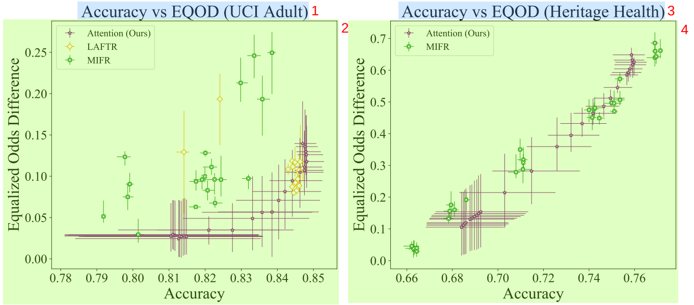
Figure 7: Accuracy vs equalized odds curves for UCI Adult and Heritage Health datasets. 5
