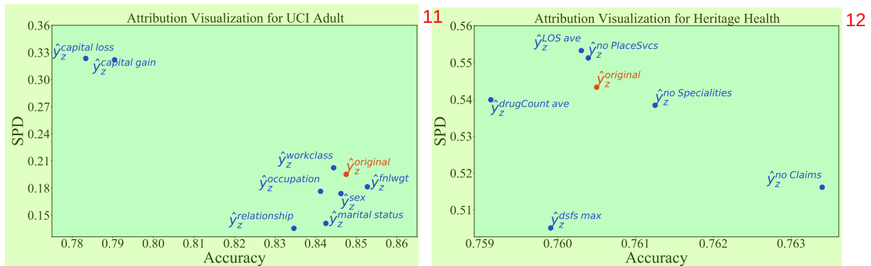
Figure 9: Results from the real-world datasets. Note that in our \hat{y}_z notation we replaced indexes with actual feature names for clarity in these results on real-world datasets as there is not one universal indexing schema, but the feature names are more universal and descriptive for this case. Labels on the points represent the feature name that was removed (zeroed out) according to our \hat{y}_z notation. The results show how the accuracy and fairness of the model (in terms of statistical parity difference) change by exclusion of each feature. 13
