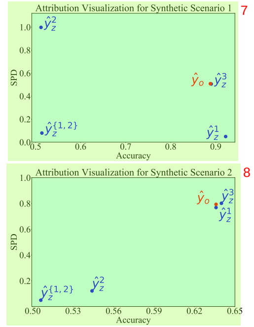
Figure 2: Results from the synthetic datasets. Following the \hat{y}_o and \hat{y}_z notations, \hat{y}_o represents the original model outcome with all the attention weights intact, while \hat{y}_z^k represents the outcome of the model in which the attention weights corresponding to k^{th} feature are zeroed out (e.g. \hat{y}_z^1 represents when attention weights of feature f_1 are zeroed out). The results show how the accuracy and fairness of the model (in terms of statistical parity difference) change by exclusion of each feature. 9
