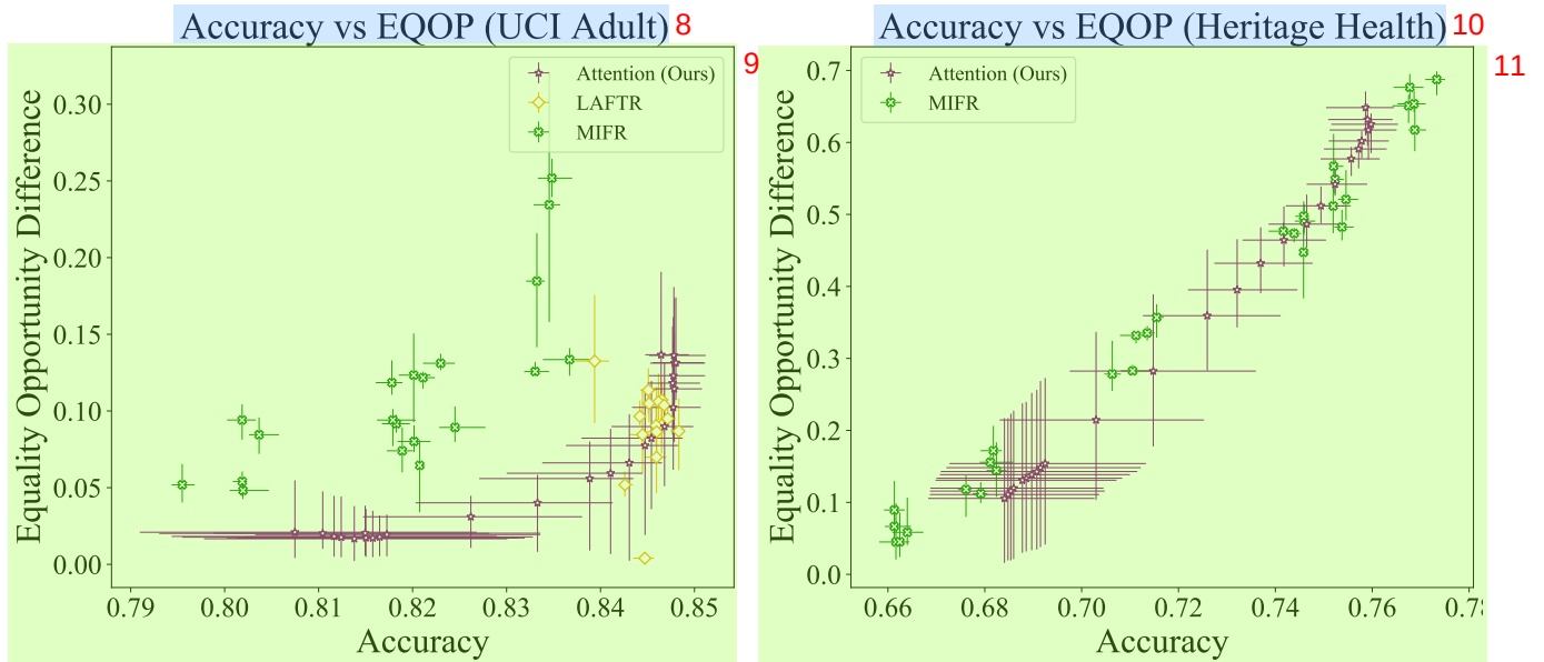
Figure 6: Accuracy vs equality of opportunity curves for UCI Adult and Heritage Health datasets. 12
