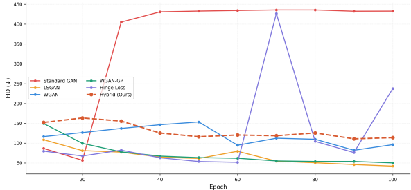
FID Curves — CIFAR-10
