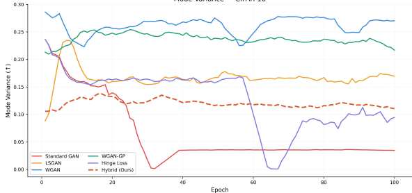
Mode Variance — CIFAR-10
