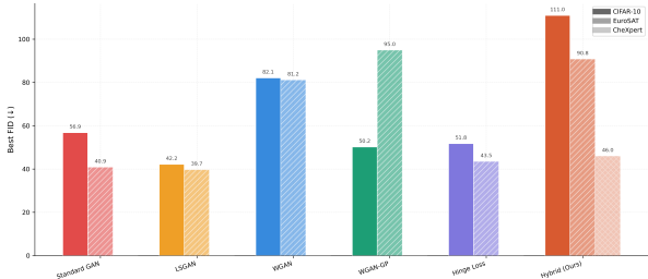
Best FID — All Datasets
