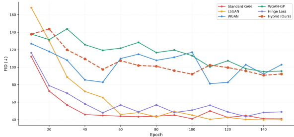
FID Curves — EuroSAT
