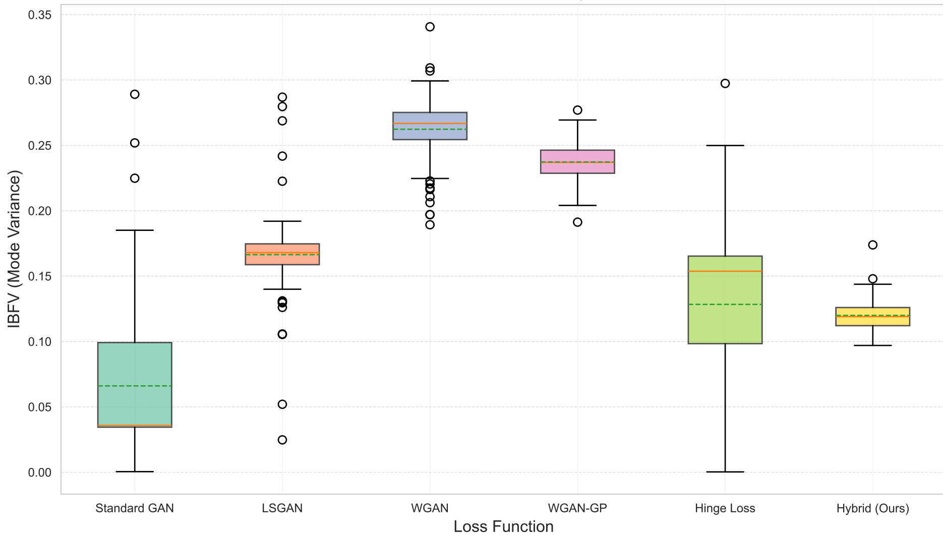
Distribution of IBFV Across Batches/Epochs on CIFAR-10
