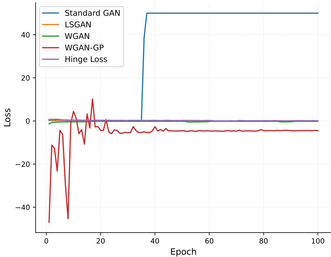
Discriminator Loss - CIFAR-10
