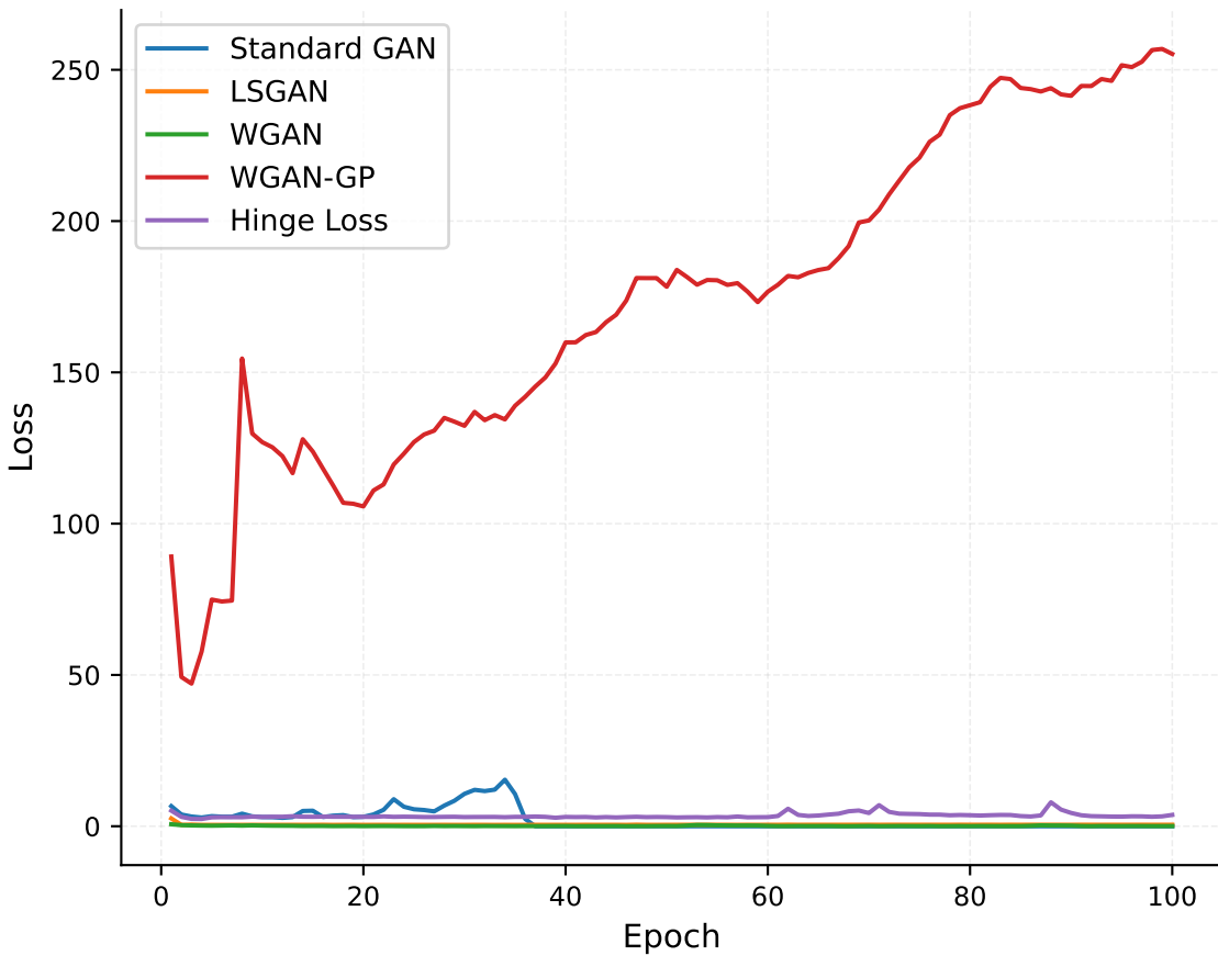
Generator Loss - CIFAR-10
