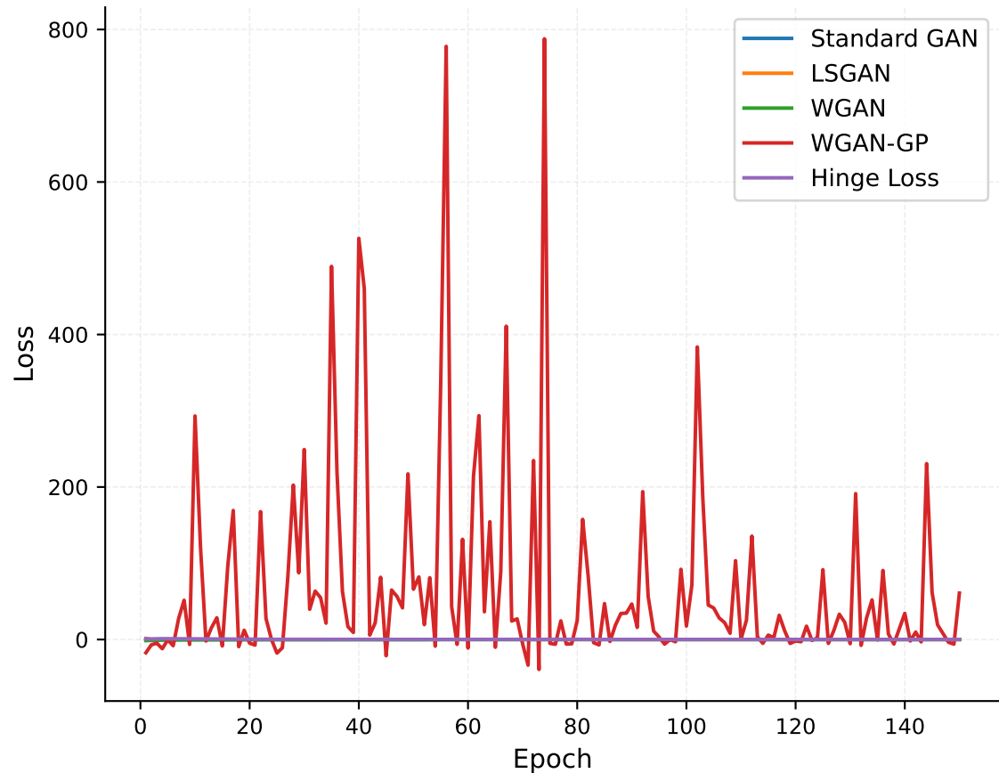
Discriminator Loss - EuroSAT
