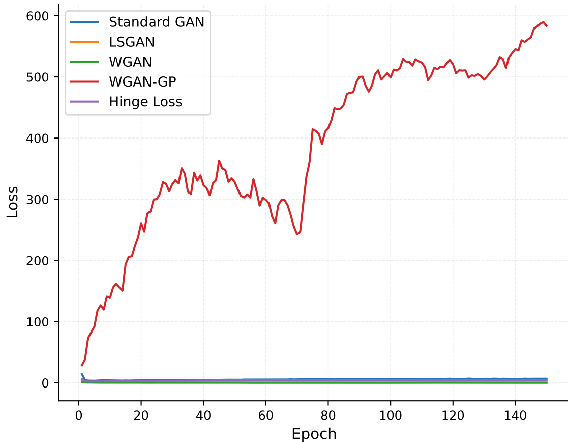
Generator Loss - EuroSAT
