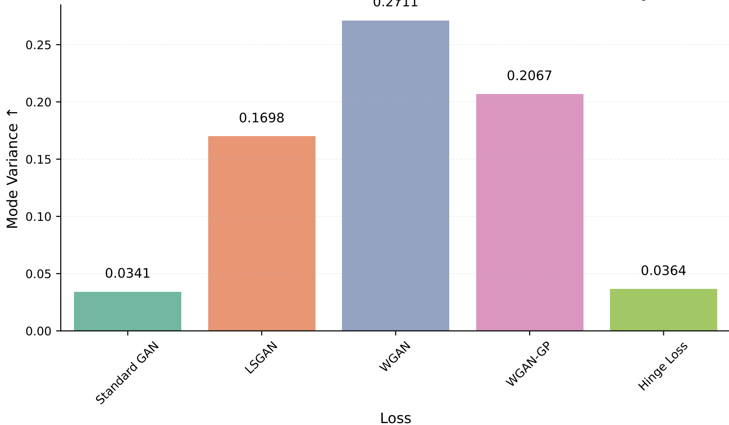
Mode Variance on CIFAR-10 (higher is better - more diversity)
