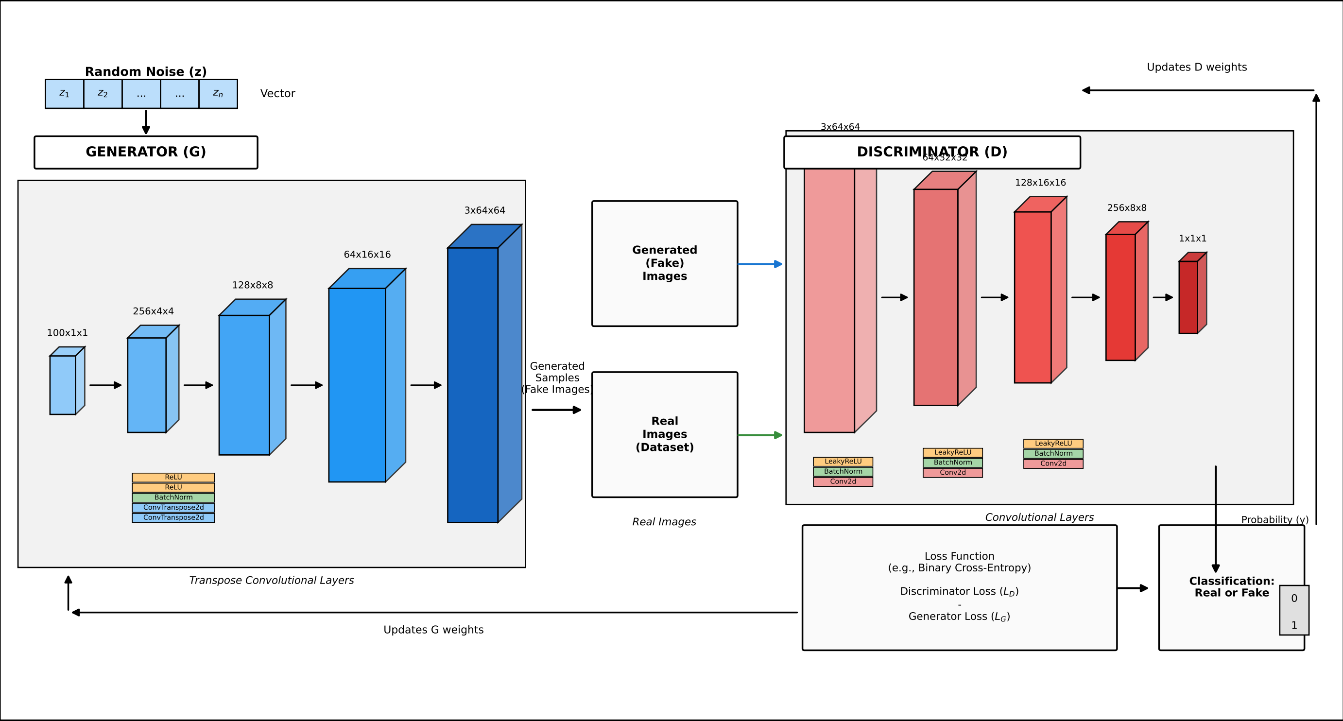
Figure 1: Architecture and Flow of the DCGAN Framework
