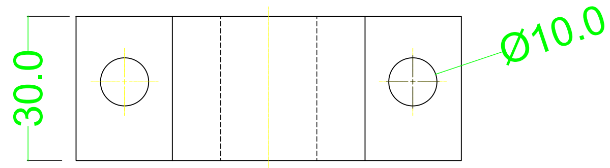
Top view
