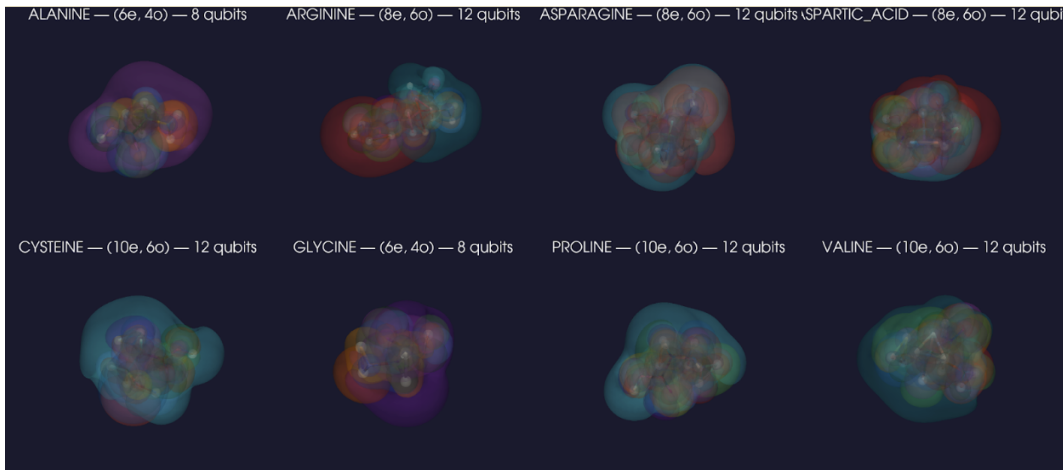
Figure 2: Active orbitals of model amino acids, visualized.
