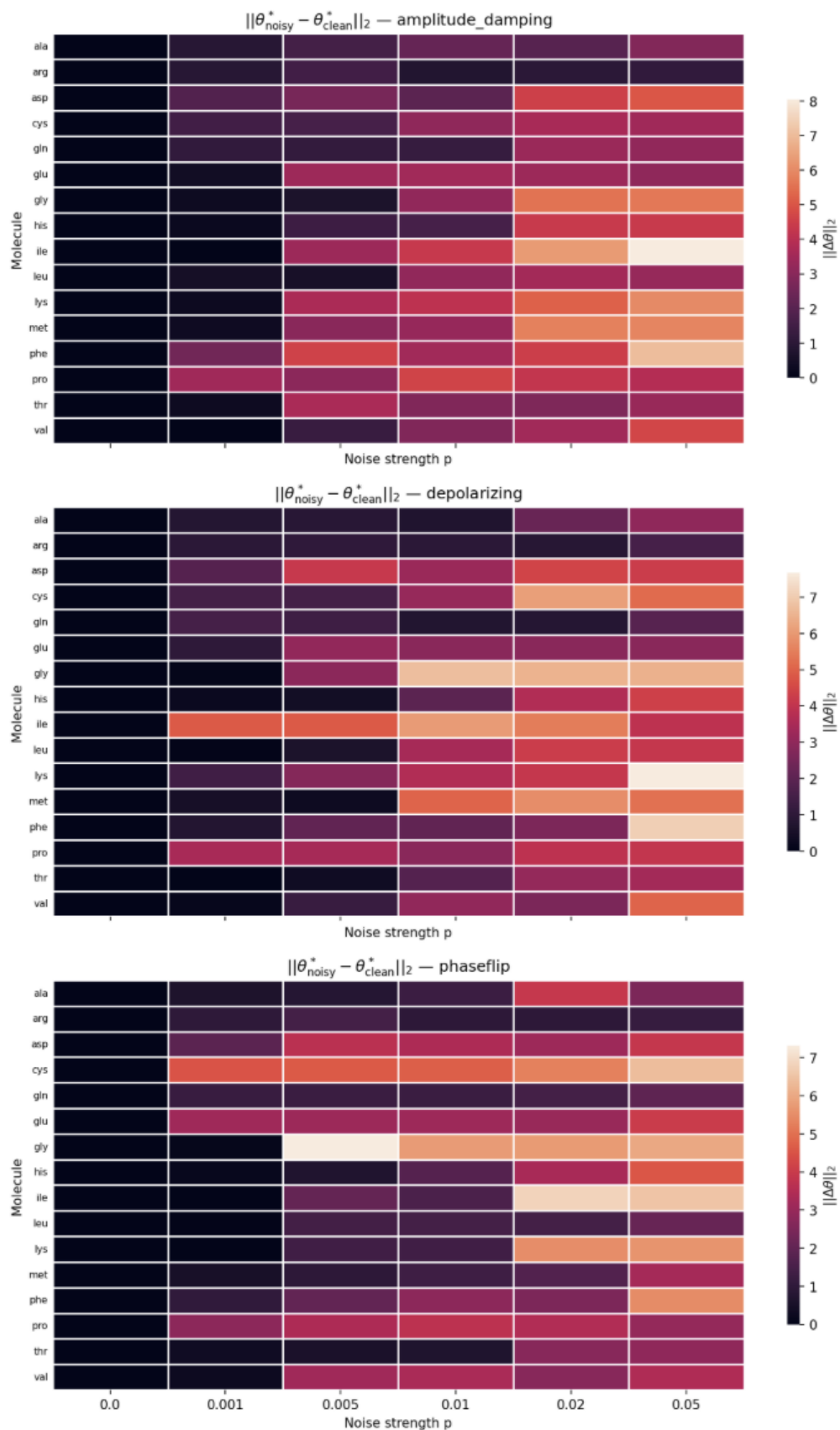
Figure 8: Heatmap of parameter drift measured using the L2 norm.
