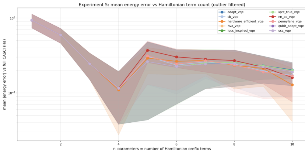
Figure 14: Investigating how much keeping the first n -parameters influences the mean energy deviation.
