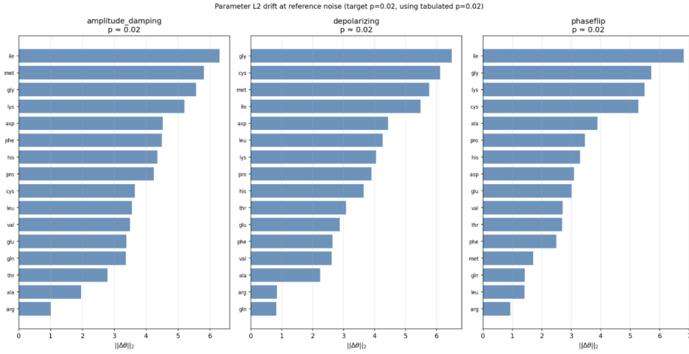
Figure 7: Parameter L2 Drift at Reference Noise. These, on their own, don’t tell you much about how significant the parameter drift is relative to baseline, but does tell you about relative drift between molecules. Refer to Figure 8 for further information. These were run on 36 parameters on 6-qubit, 2-layer RY hardware-efficient setup; an L2 norm of roughly 6 is compatible with “order-1 radian” average coordinate shifts. This was generated from experiment 1.
