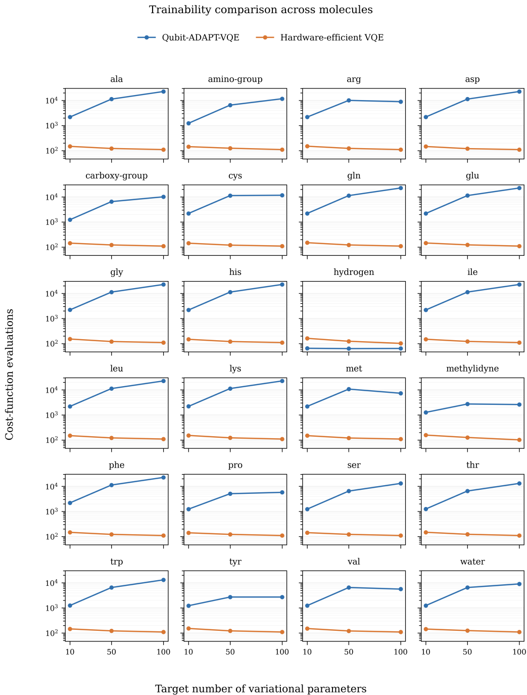
Figure 13: Cost-function evaluations required by Qubit-ADAPT-VQE and hardware-efficient VQE across the trainability benchmark molecules. Each panel shows one molecule, with evaluations plotted on a logarithmic scale against the target number of variational parameters.
