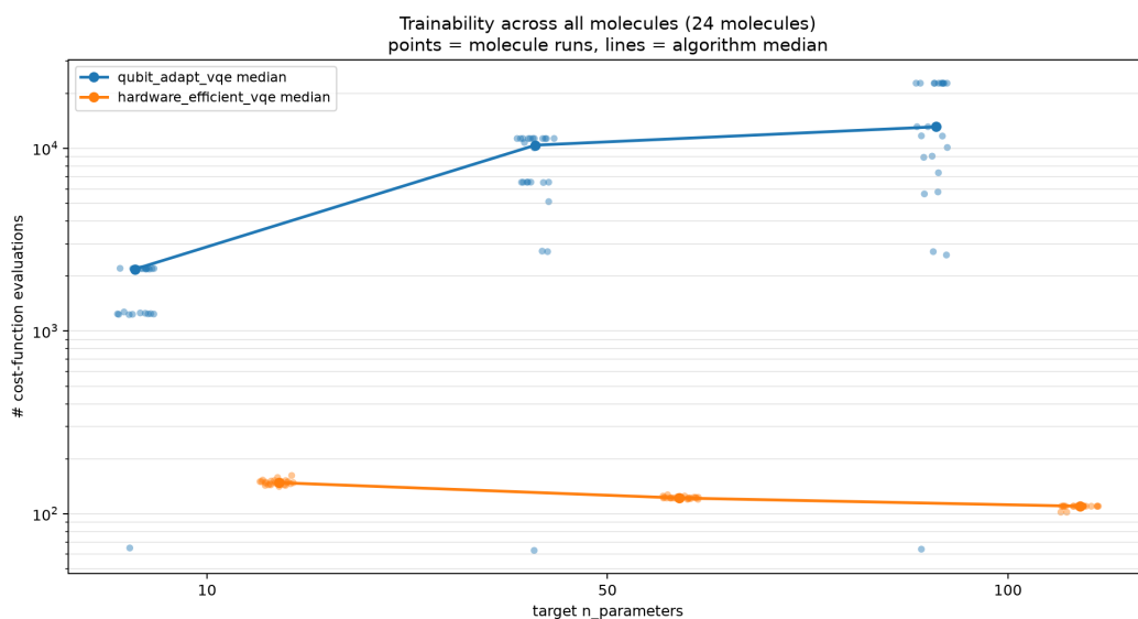
Figure 12: Investigating cost-fn evals for all molecules between qubit-ADAPT and hardware-efficient VQE.
