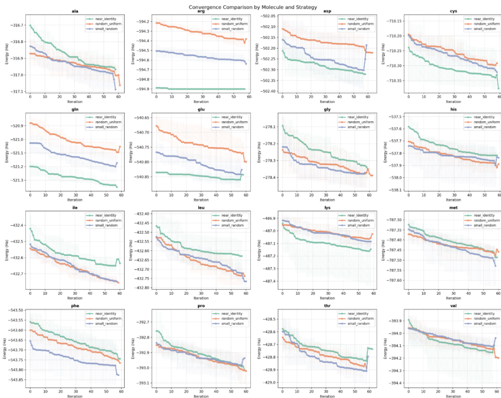
Figure 9: Investigating convergence for different strategies for amino acids from the dataset, using hardware_efficient_vqe .
