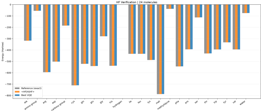
Figure 3: HF Verification VS other metrics on the 24 QMProt molecules.
