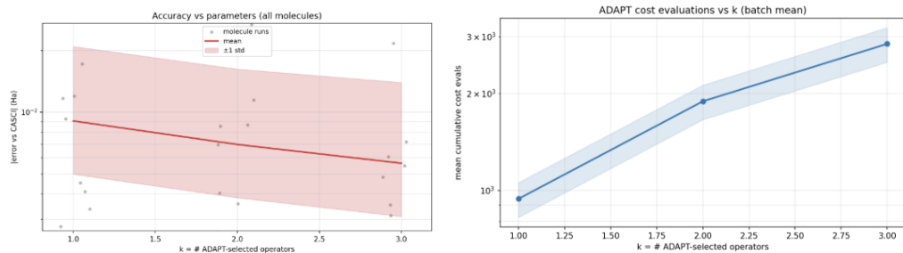
Figure 11: Investigating energy error vs n_{\text{parameters}} for Adapt-VQE, compared to the CASCI. All of the amino acids in the QMProt dataset were run up to k = 3 . Larger experiments can be run.
