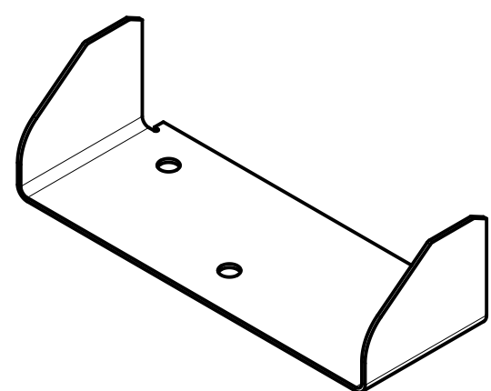
REFERENCE ISOMETRIC VIEW SCALE 1:6
