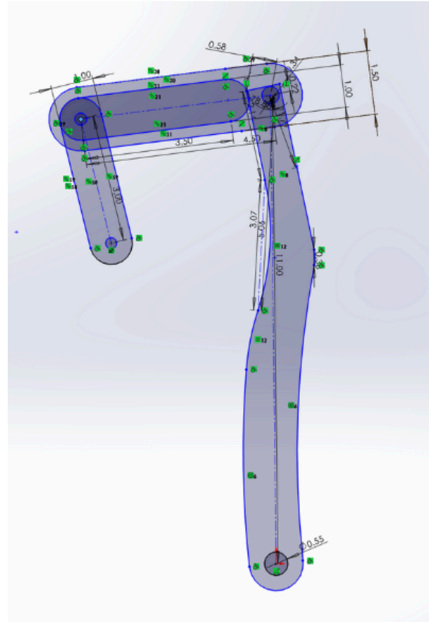
Early Concept for Actuating Brake Pedal In Place of Extra Master Cylinder Approach
