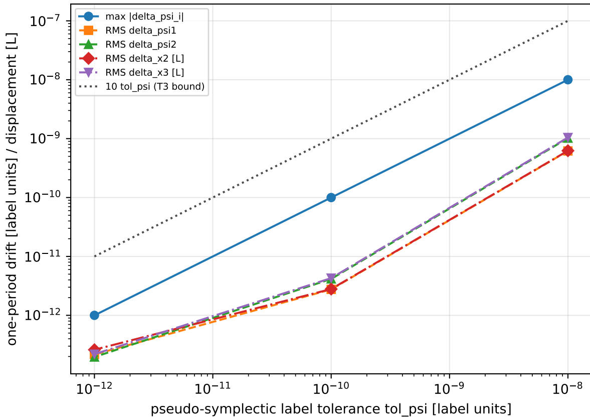
analytic_G_a0.05_n128 (label route: analytic): pseudo-symplectic drift
