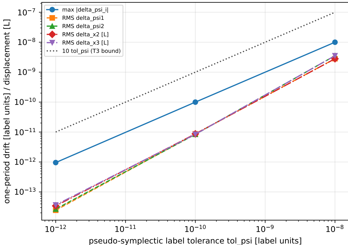
stack_lester2021_e0.25_n128 (label route: stack): pseudo-symplectic drift
