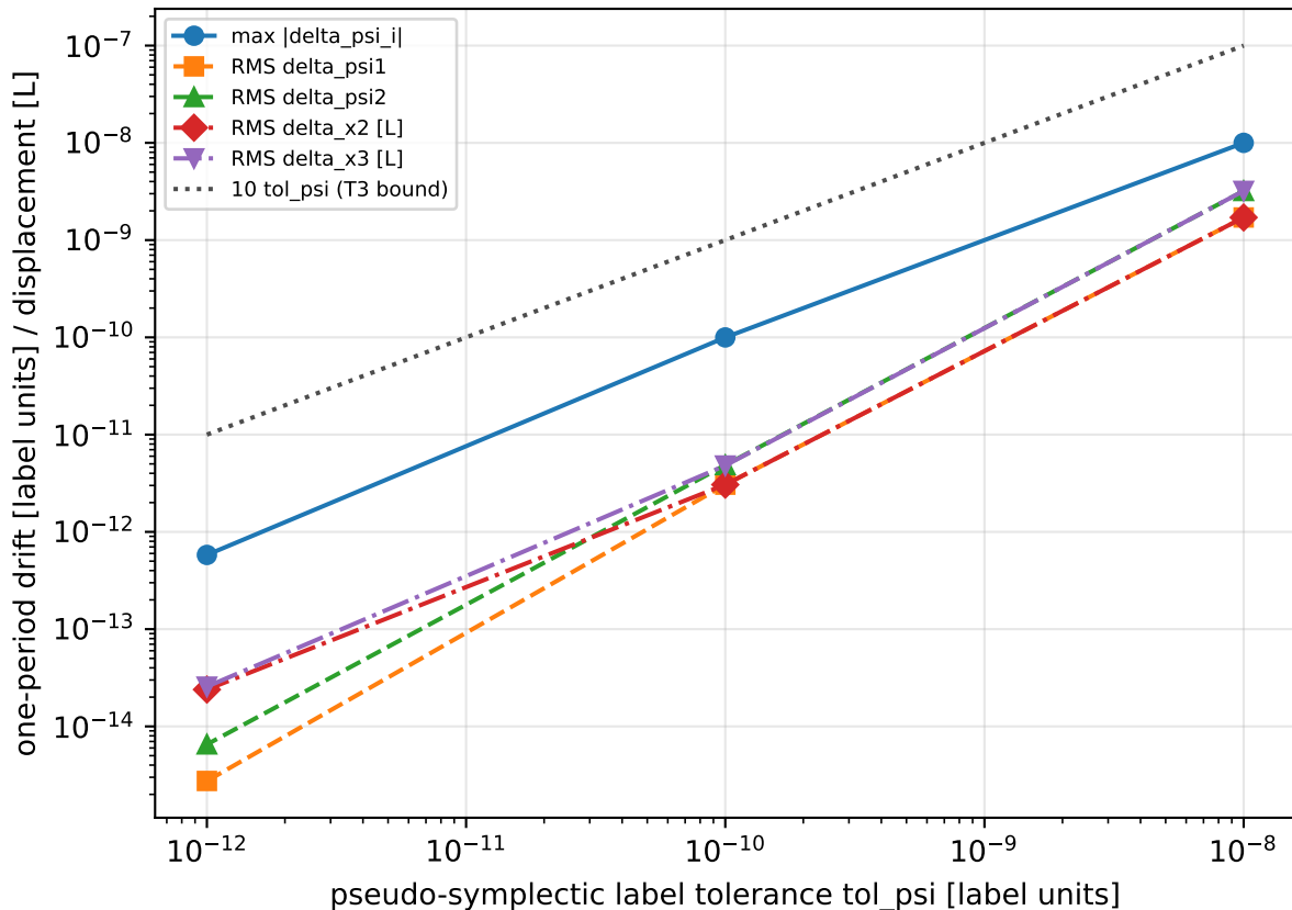
stack_lester_brk_e0.25_n256 (label route: stack): pseudo-symplectic drift
