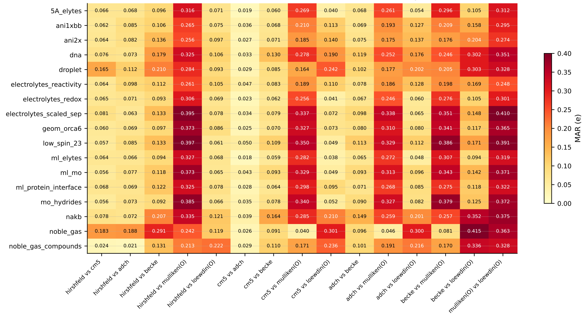
Charge-scheme MAR per vertical x scheme-pair (17 verticals) median absolute residual across atoms; lower = better cross-scheme agreement
