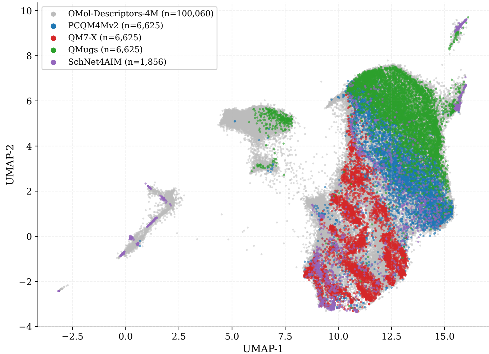
SOAP UMAP: OMol-Descriptors-4M vs Structural Comparators
