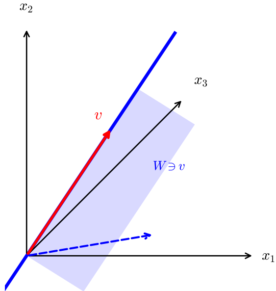
(b) Type 2: Stoichiometric first integral
