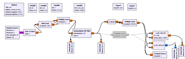
Figure 5. Block diagram for FSK modulation for a bipolar signal.
