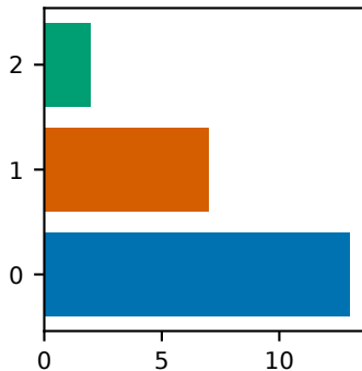
Extraction strategy
