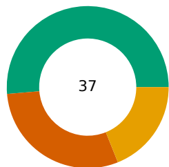
Extraction strategy
