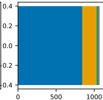
SSSOM predicates
