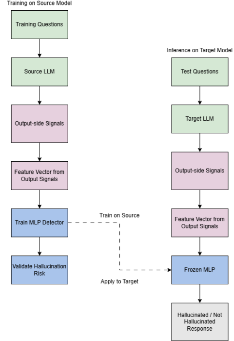
Figure 2. Overview of the proposed output-side hallucination detection pipeline. Each model answers the same Common-senseQA questions, responses are labeled using ground truth answers, output-side features are extracted from generation, and an MLP detector is evaluated under same-model, cross-model, and pooled-training settings.
