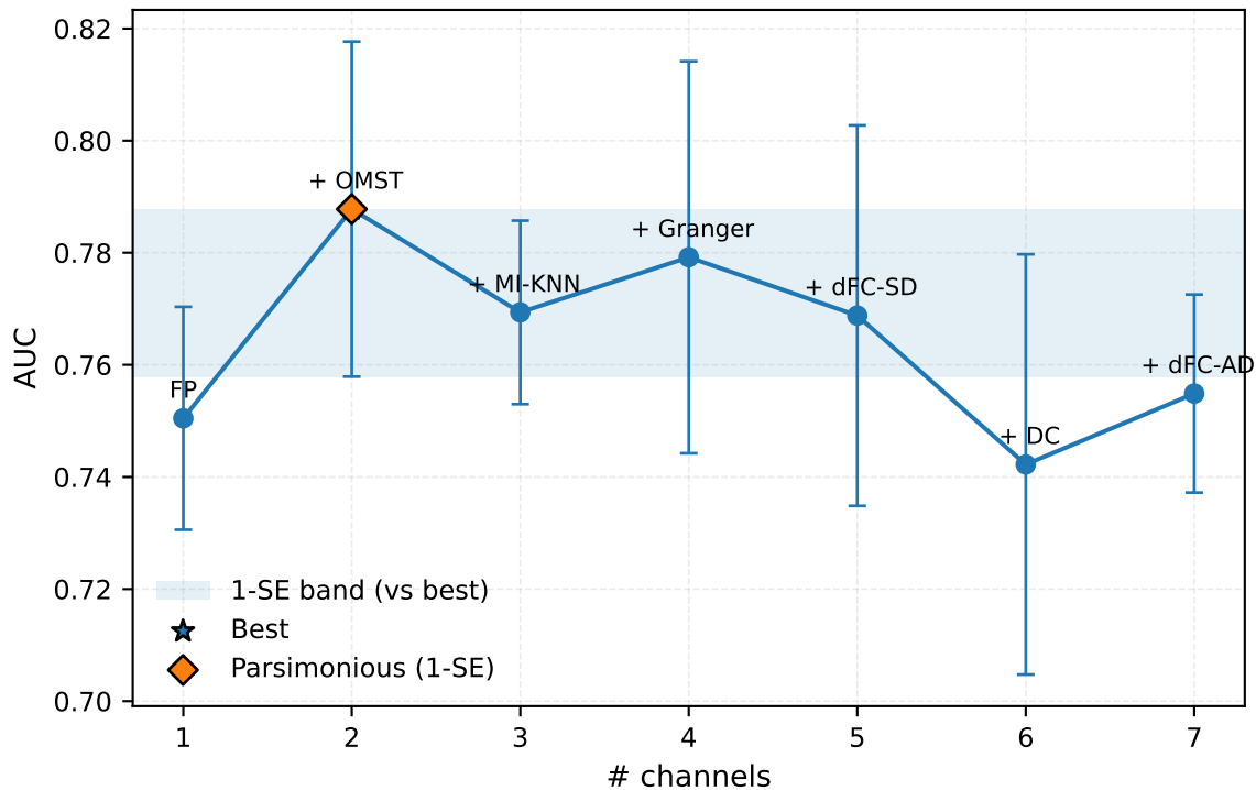
Ablation curve: performance vs #channels
