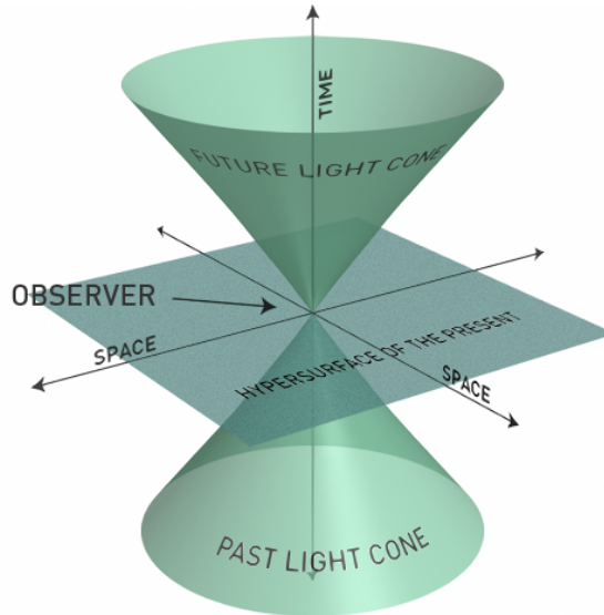
Figure A.1: Representation of a light cone
