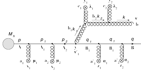
Figure 3.18: Diagram for gluon propagation inside the medium with two scatterings.
