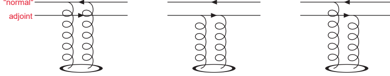
Fig. 4. Different contributions to the dipole cross section
