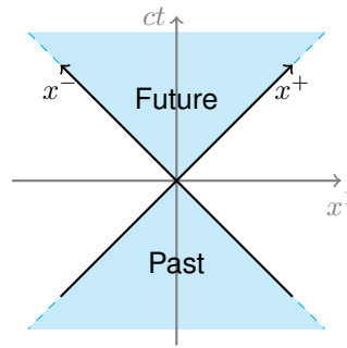
Figure A.1: Position four-vector axes in light-cone coordinates.
