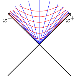
Figure A.2: Contour lines for proper time, \tau , in red, and rapidity, \eta , in blue, in the first quadrant.
