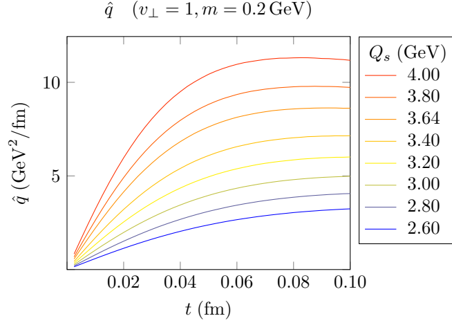
Figure 5.4: \hat{q}(t) for several values of Q_s . Since v_{\parallel} = 0 , t = \tau .
