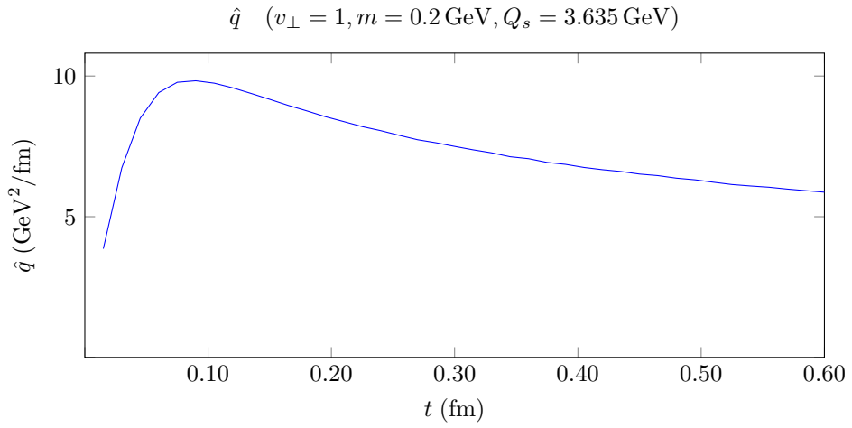
Figure 5.12: \hat{q} up to t = 0.6 \text{ fm} . Since v_{\parallel} = 0 , t = \tau .
