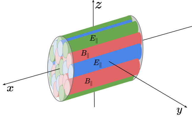
Figure 2.8: The “glasma flux tube” picture of the early glasma ( \tau \rightarrow 0^+ ). Right after the collision, the space between the receding nuclei is populated by purely longitudinal chromoelectric and chromomagnetic fields, whose direction lies along the drawn tubes. Adapted from [15].
