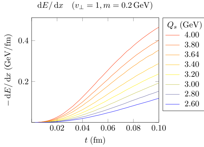
Figure 5.5: dE/dx for several values of Q_s . Since v_{\parallel} = 0 , t = \tau .
