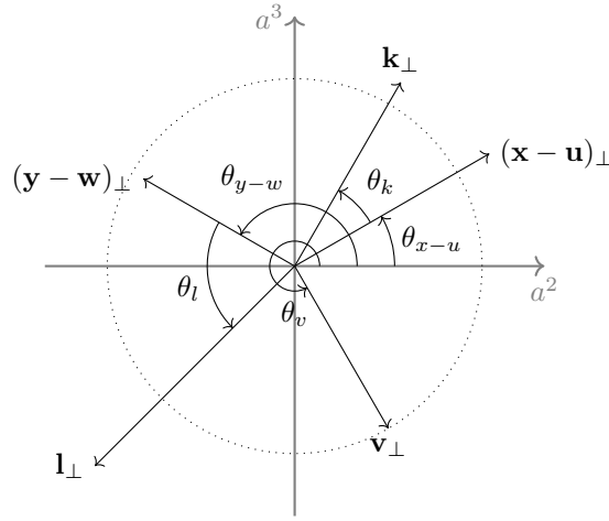
Figure C.1: Relative positions and angles defined between the vectors (\mathbf{x} - \mathbf{u})_\perp , (\mathbf{y} - \mathbf{w})_\perp , \mathbf{k}_\perp , \mathbf{l}_\perp and \mathbf{v}_\perp at some point in the integration.
