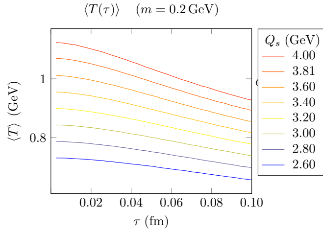
Figure 5.3: \langle T(\tau) \rangle for several values of Q_s .
