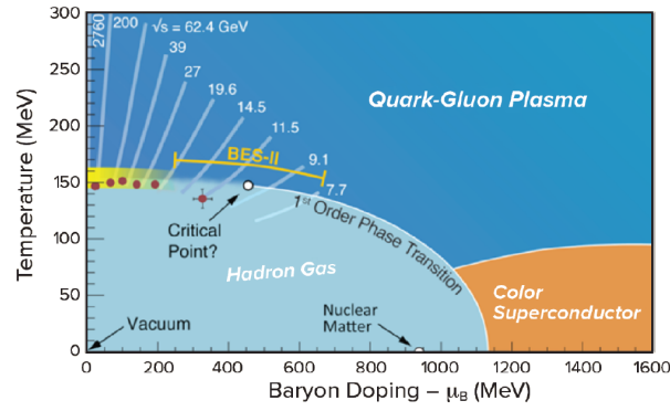
Figure 1.6: A possible QCD phase diagram. Also shown are lines representing the path drawn by cooling QGP droplets from HICs at different \sqrt{s} and expected paths from the then-upcoming phase II of RHIC's Beam Energy Scan. From [3].
