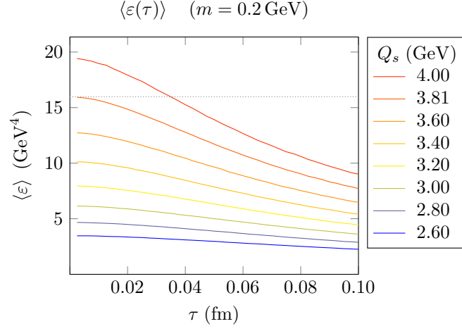
Figure 5.1: \langle \varepsilon(\tau) \rangle for several values of Q_s . Dotted in gray, [15]’s value for the initial energy density, \langle \varepsilon_0 \rangle = 15.9773 \text{ GeV}^4 ; it matches this work’s initial energy density for Q_s \approx 3.8079 \text{ GeV} .
