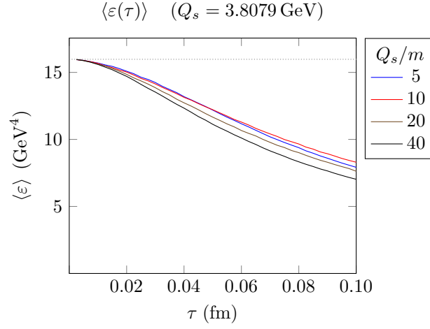
Figure 5.2: \langle \varepsilon(\tau) \rangle for several values of Q_s/m .
