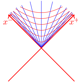
Figure B.1: Position four-vector axes in light-cone coordinates.
