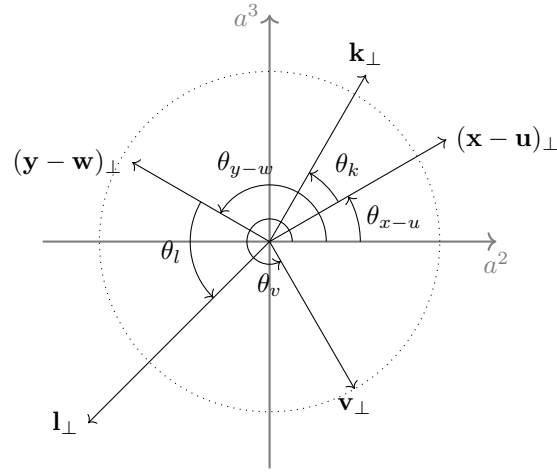
Figure 4.1: Relative positions and angles defined between the vectors (\mathbf{x} - \mathbf{u})_\perp , (\mathbf{y} - \mathbf{w})_\perp , \mathbf{k}_\perp , \mathbf{l}_\perp and \mathbf{v}_\perp at some point in the integration.
